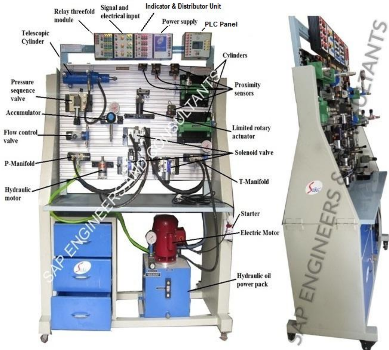
ADVANCED CUSTOMIZED ELECTRO-HYDRAULIC TRAINER (SAP-38 D)
